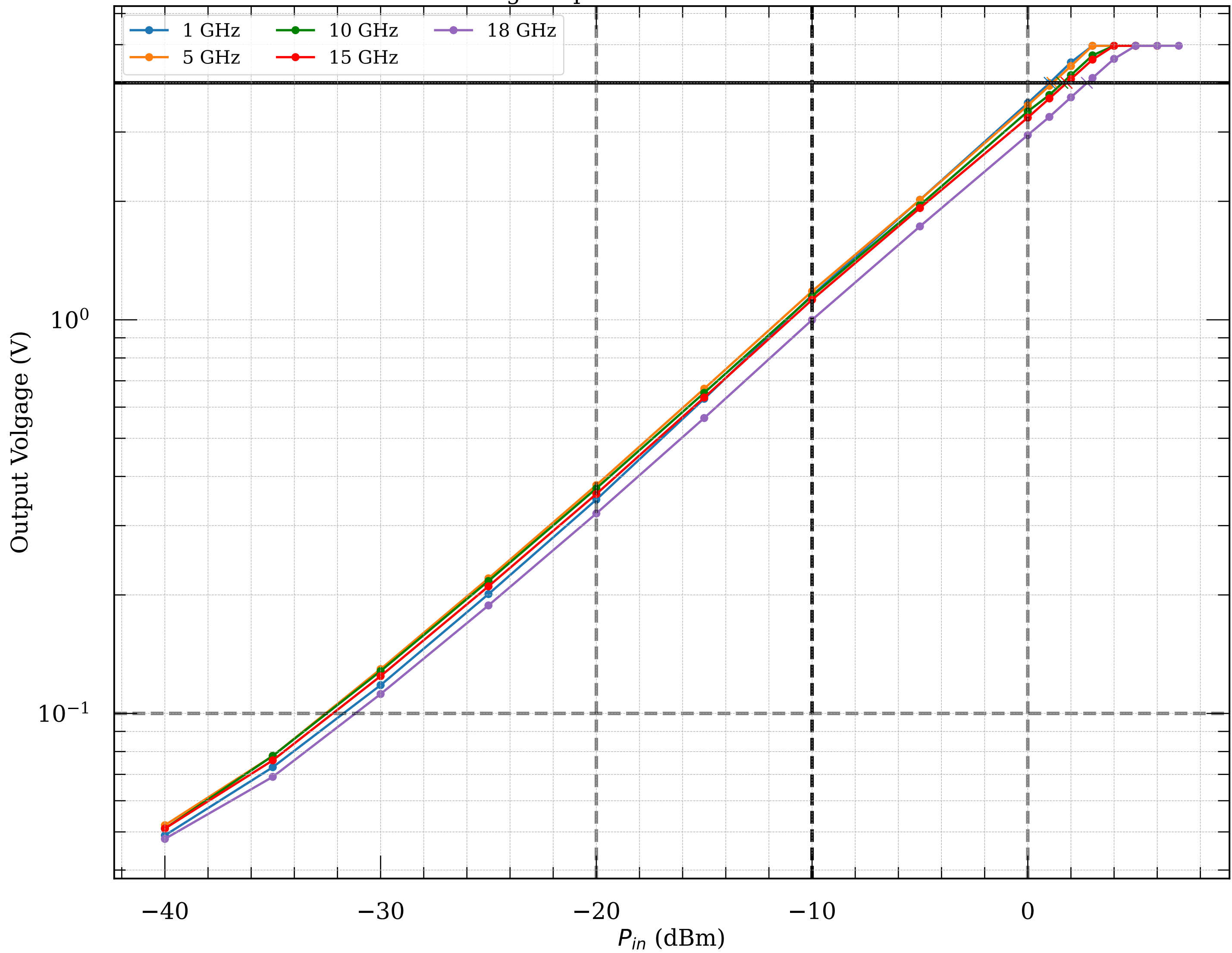
Measured voltage-to-power curve of detector module046v2
